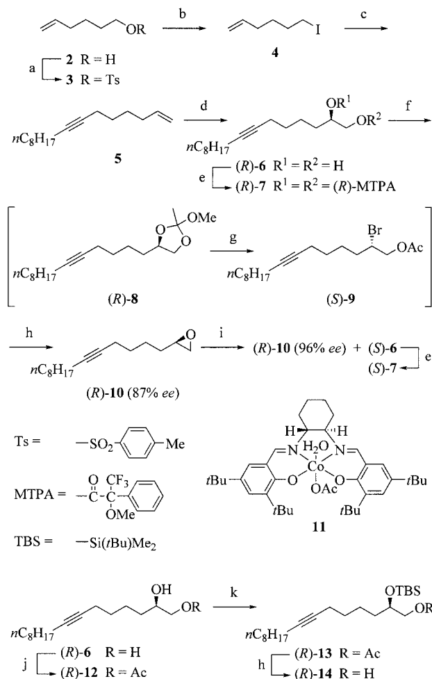
Scheme 2. Synthesis of ( R )-1,2-epoxyhexadec-7-yne ( 10 ). Reagents: (a) TsCl, C 5 H 5 N; (b) NaI, DMF (92%, 2 steps); (c) C 8 H 17 C \equiv CH, n BuLi, THF (71%); (d) AD-mix- \beta , t BuOH, H 2 O, 0–5 °C, 6 h, then room temp. overnight; recrystallization from hexane [1 \times (84%) for ( R )- 6 of 75% ee ; 2 \times (60%) for ( R )- 6 of 87% ee ; 5 \times (20%) for ( R )- 6 of 98% ee ]; (e) ( S )-MTPACl, DMAP, C 5 H 5 N; (f) MeC(OMe) 3 , PPTS, CH 2 Cl 2 ; (g) AcBr, CH 2 Cl 2 ; (h) K 2 CO 3 , MeOH [87% for ( R )- 10 , 3 steps; quant. for ( R )- 14 ]; (i) Jacobsen's ( R,R )-salen cobalt catalyst ( 11 ), 0.4 equiv. H 2 O, THF [72% of ( R )- 10 (96% ee ) and 20% of ( S )- 6 (49% ee )]; (j) lipase PS, CH 2 =CHOAc, i Pr 2 O (99%); (k) TBSCl, imidazole, DMF (86%).
