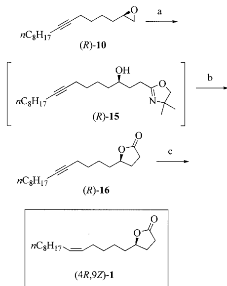
Scheme 3. Synthesis of (4R,9Z)-octadec-9-en-4-olide (1). Reagents: (a) 2,4,4-trimethyl-2-oxazoline, n BuLi, THF, -78^{\circ}\text{C} to room temp.; (b) dil. HCl, THF, 60^{\circ}\text{C} , 30 min (58%, 2 steps); (c) \text{H}_2 , Lindlar Pd– \text{CaCO}_3 – \text{Pb}^{2+} , hexane, -5 to 0^{\circ}\text{C} (94%).
